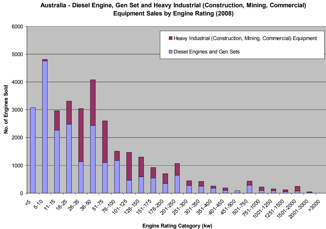
Figure 10: Diesel engine, gen set and heavy industrial equipment sales (2008) by engine rating Data Source: ERG International, 2009
