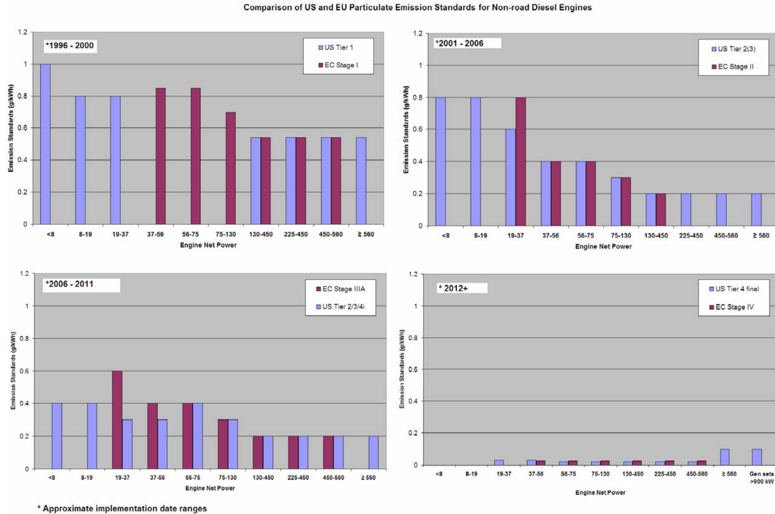
Figure 5: Comparison of US and EU emission standards for non-road diesel engines (particulate matter)
