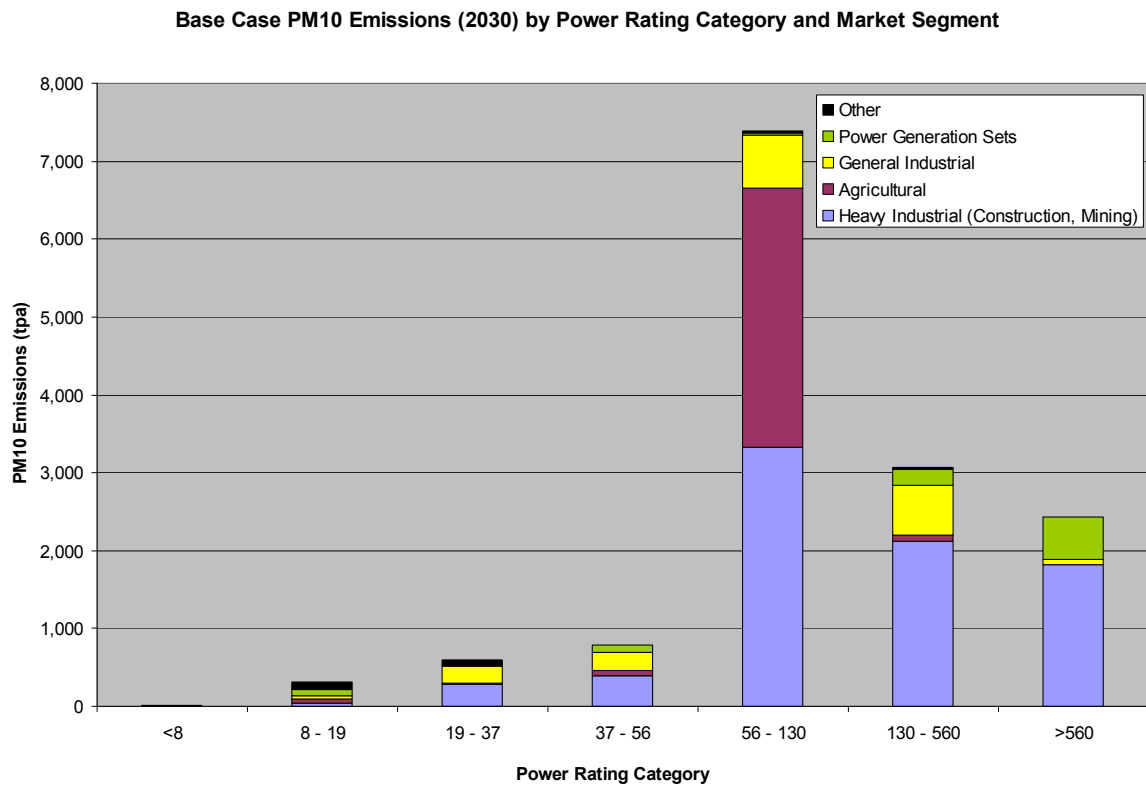
Figure 24: Upper Bound Base case PM 10 emissions from non-road diesel engines for 2030 by power rating and market segment
