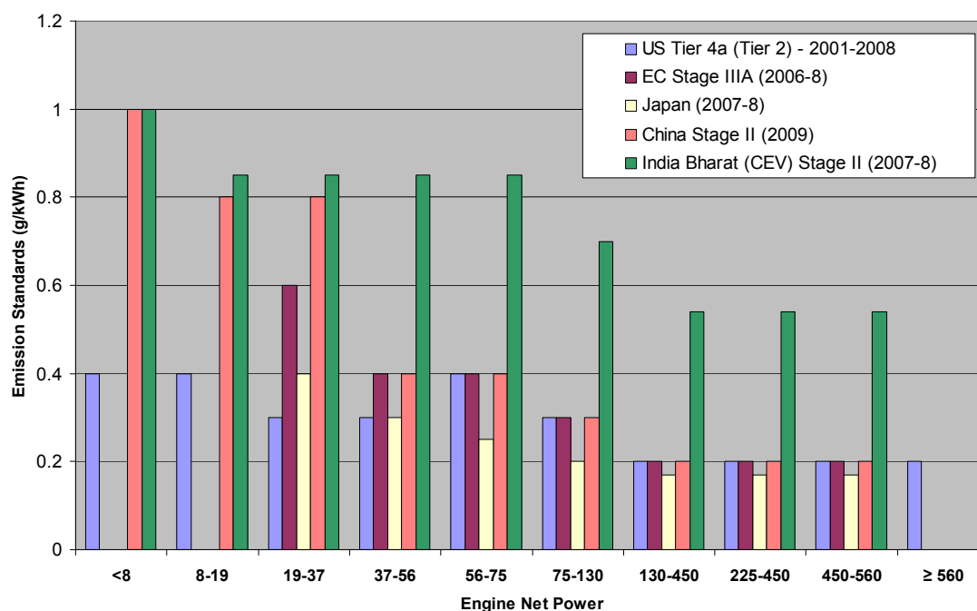
Figure 6: Comparison of particulate matter emission standards for non-road diesel engines published by the US, EC, Japan, China and India for implementation prior to 2010.
