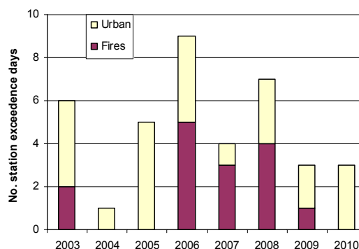
Figure 5: Inferred causes of exceedances of the PM_{2.5} 24-hour standard (Port Phillip region 2003-10)
