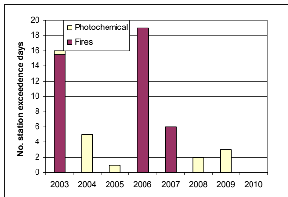
Figure 3: Inferred causes of exceedances of the ozone four standard (Port Phillip region 2003-10)
