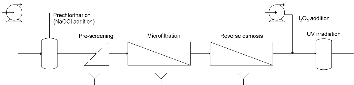
Figure 3-15: Advanced Water treatment – process flow diagram
