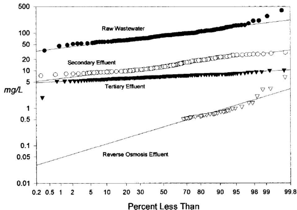
Figure 3-12: Log normal cumulative probability plot for TOC after various treatment processes (Eisenberg et al. , 2001).
